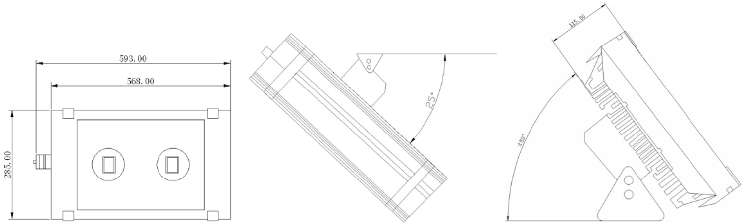
Figure 6. Mechanical Dimensions
